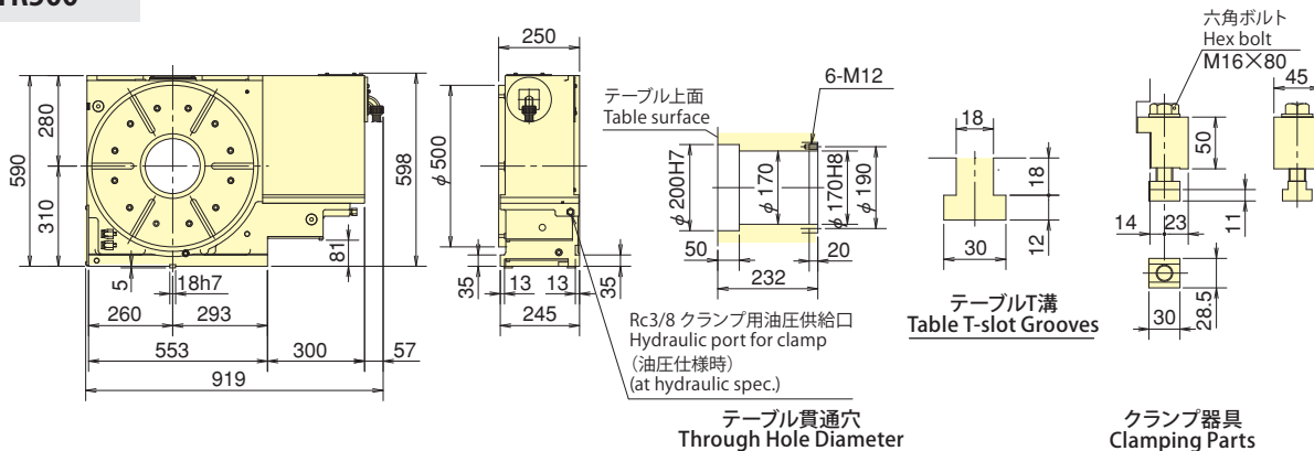
TR500
