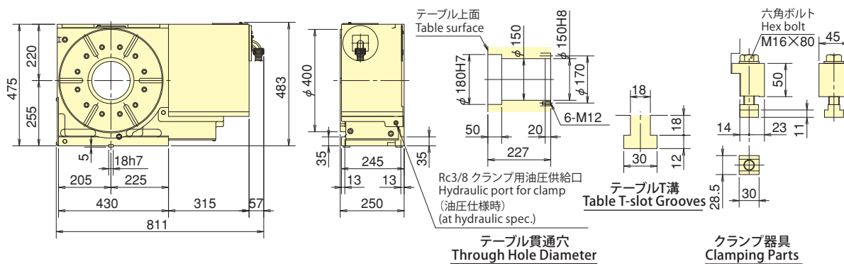
TR500
