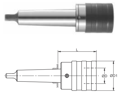
Morse Taper Style
