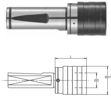
Straight Shank W/ Modular Shank
