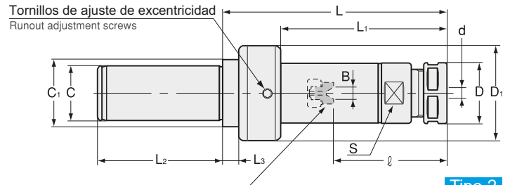
Tornillo de preajuste (incluido) Preset Screw (included)
