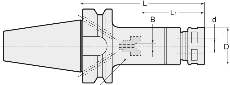
Tornillo de preajuste (incluido) Preset Screw (Included)
