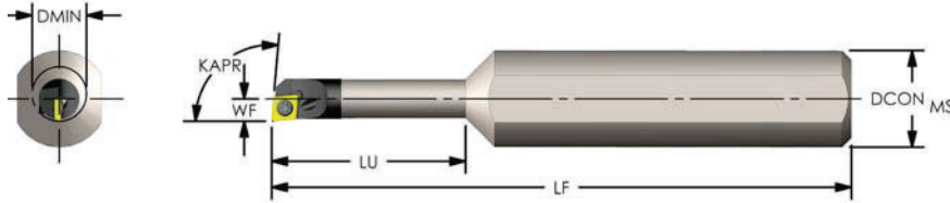
Positive 80° Diamond (KAPR: 95°) Reduced Neck SERIES "C"
