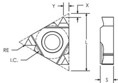
Partial Profile 60°
