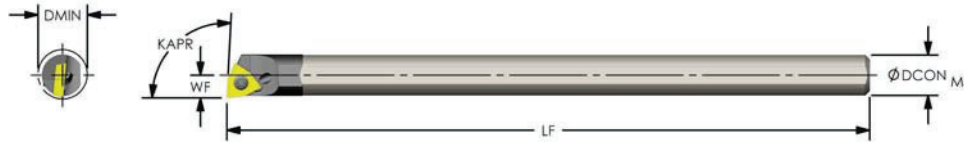
Positive Trigon (KAPR: 93°) SERIES "G, Q, S"
