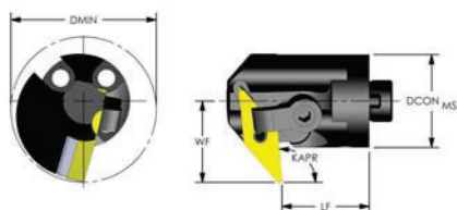
Negative 35° Diamond ( KAPR: 95°) Back Facing
