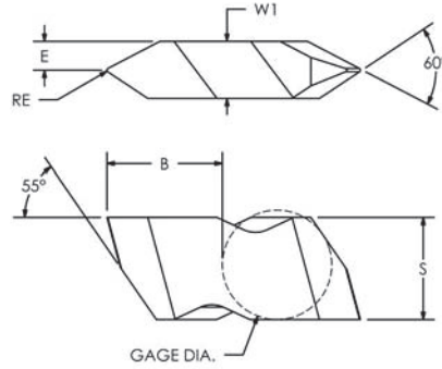
Top Notch Threading
