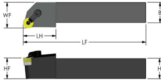
Negative Round (0° Lead)
