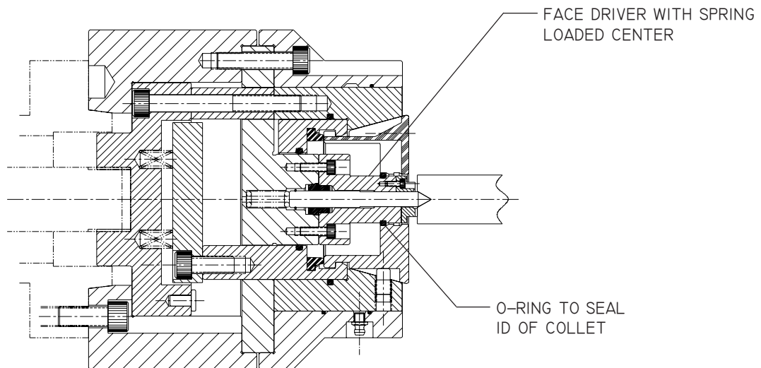
COLLET RETRACTED
